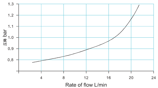
Pressure graph
