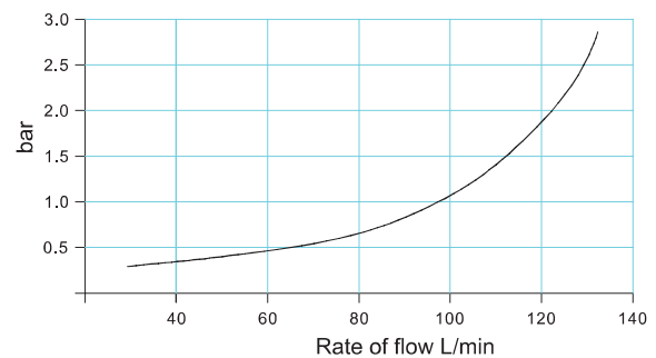
Pressure graph
